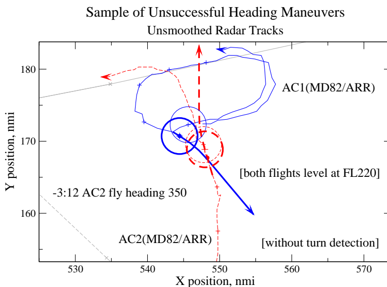
Figure 8. Unsmoothed radar tracks for a sample operational error that was not resolved in simulation by heading maneuvers (both flights level at FL220)
