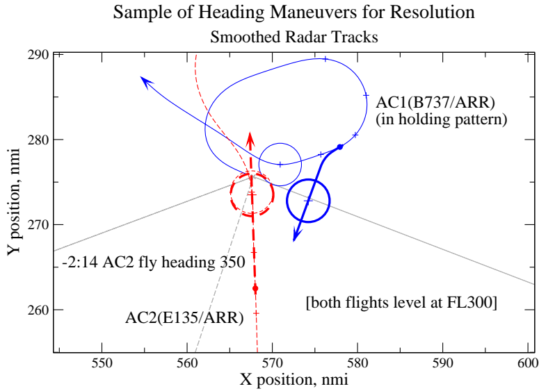
Figure 6. Smoothed radar tracks for a sample operational error that was resolved in simulation by heading maneuvers (both flights level at FL300)
