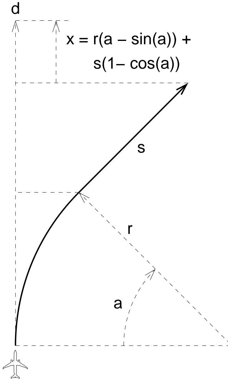
Figure 3. Geometry for computation of extra distance flown due to a heading maneuver
