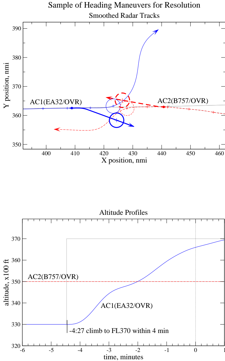
Figure 5. Smoothed radar tracks (top) and altitude profiles (bottom) for a sample operational error that was resolved in simulation by heading maneuvers
