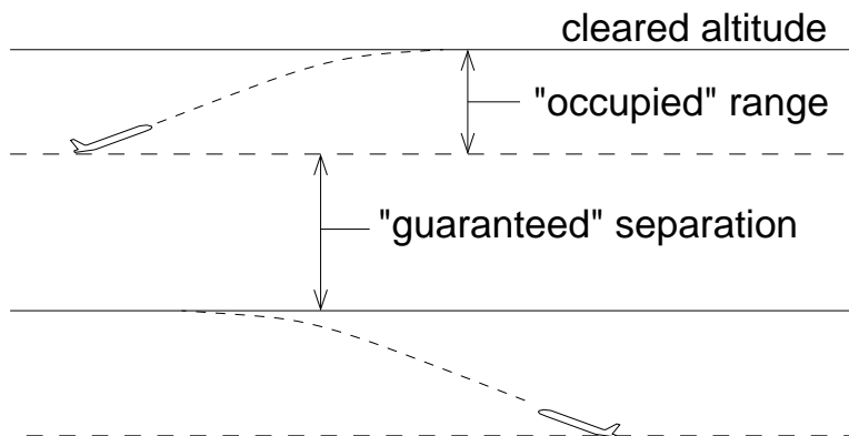
Figure 2. The encounter separation ratio does not apply when the flights are “separated by altitude clearance” (i.e., the “guaranteed” separation is greater than or equal to the minimum required separation)
