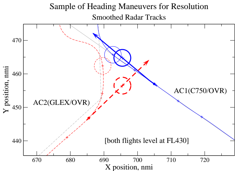
Figure 7. Smoothed radar tracks for a sample operational error that was resolved in simulation by heading maneuvers (both flights level at FL430)
