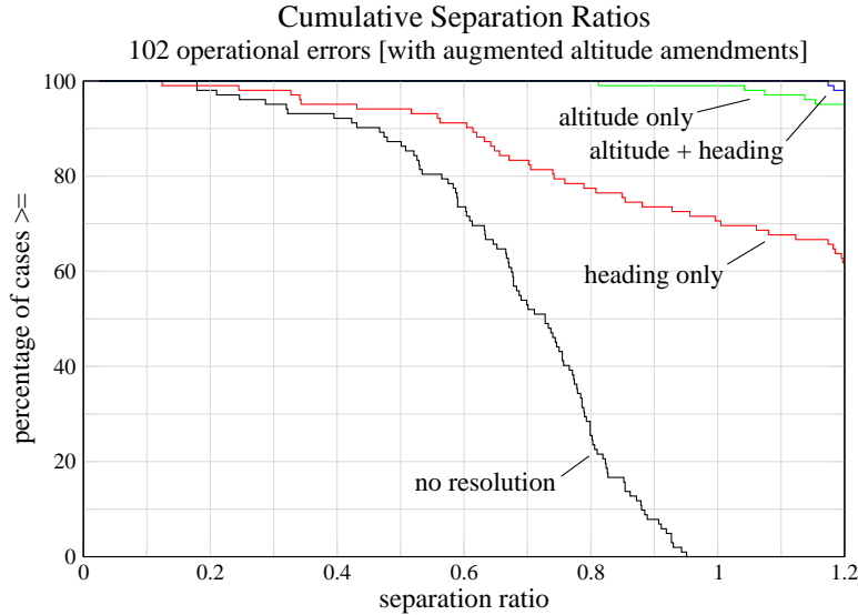
Figure 10. Cumulative separation ratio as percentage of archived operational error cases (with augmented altitude amendments)
