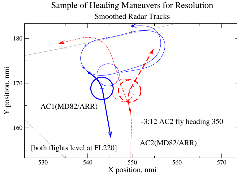
Figure 9. Smoothed radar tracks for a sample operational error that was not resolved in simulation by heading maneuvers (both flights level at FL220)
